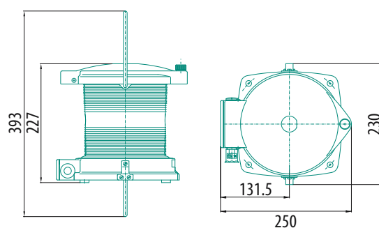
Single Lantern – hoistable
